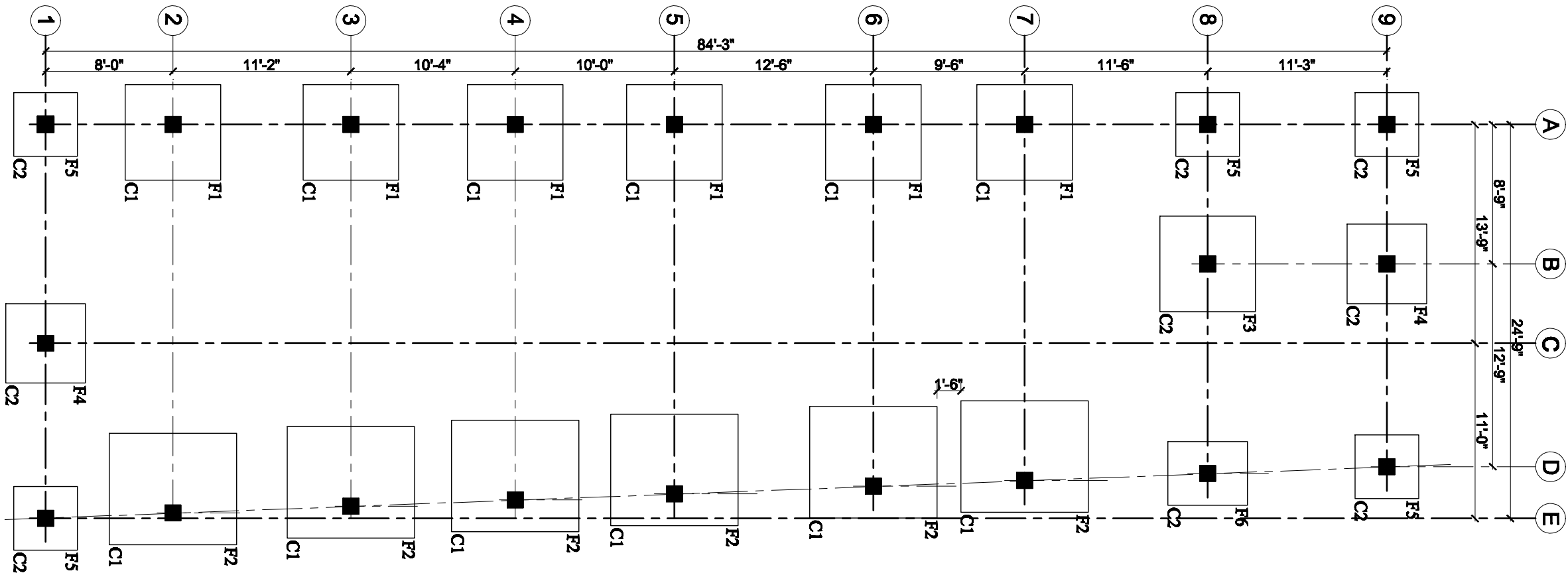
FOOTING LAYOUT
